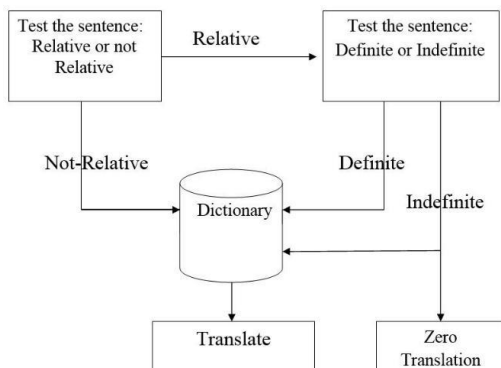
Figure (1) The Program Structure
